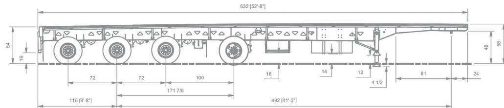
ELEVATION VIEW
